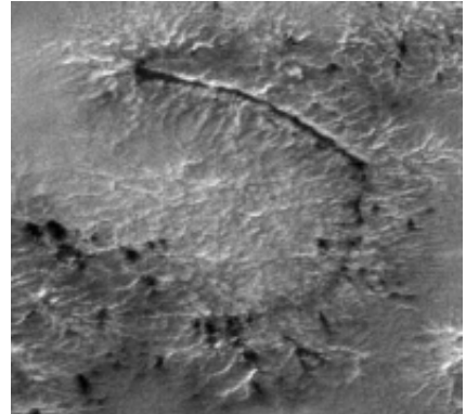
Fig. 5c Ice or snow are deposited in the edge of the fissure.
