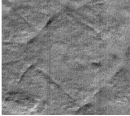
Fig. 8a Polar linear mounds in joints and faults.
