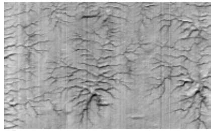
Fig. 10a 194.74°W, 76.92°S. Complex branching spiders, each around 800 m wide.
