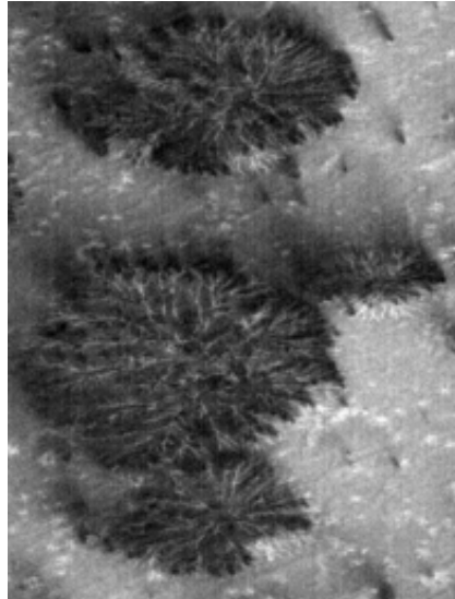
Fig. 2b 284.38°W, 82.02°S. Scale: 2.83 km across image. Bush shapes in M0804688 vent gas bubbles and dust/mud so are sometimes covered in a CO 2 fog. The Banyon Tree or bush form typically grows as a complex structure with interlocked branches, out from a central point.
