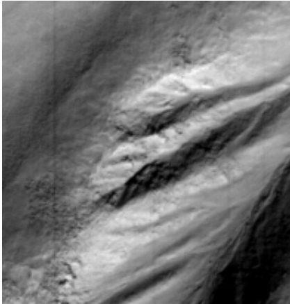
Fig. 8g Sand hills forming alluvial fans that adopt reverse drainage patterns at the South Pole. These form by growth at the toes and also down the middle of the ridge.
