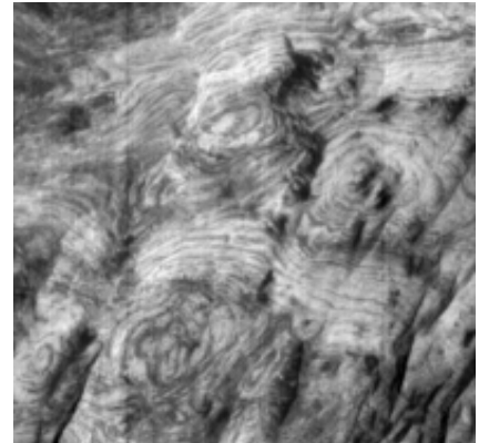
Fig. 8d (left), 8e (middle) and 8f (right) 62.08°W, 3.74°S. Each ~1.74 km wide. Late spring. Trough-cross bedded (TCB) terraces of light and dark material have formed from venting of material (possibly clathrates or ice and eroded bedrock minerals) via faults. The beds are not folded; it is the same rock unit in a continuous sequence.
