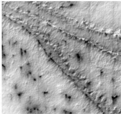
Fig. 4e 10.06°W, 79.85°S Spring. 1.42 km wide. Fans (dark) and small spiders form along the banding.
