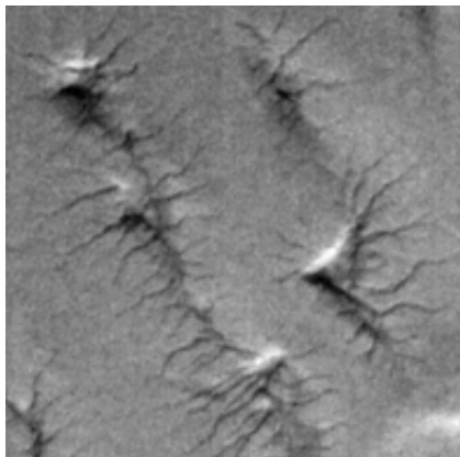
Fig. 2d Spiders reverting to ravines. Compare this to M0700604 (187.37°W, 73.69°S) where ravines have a rotated creek system and a central core with mud-like material covering the openings in the bottom of the ravines, developing tubes.
