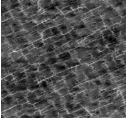
Fig. 5d Local joint patterns control.
