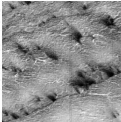
Fig. 5e Local joints and fissures control spider growth. The pale albedo (white) tubes are old spiders partly eroded by outflow channels where fluids have burst the spider. Note the plug in the fissure with vents either side.
