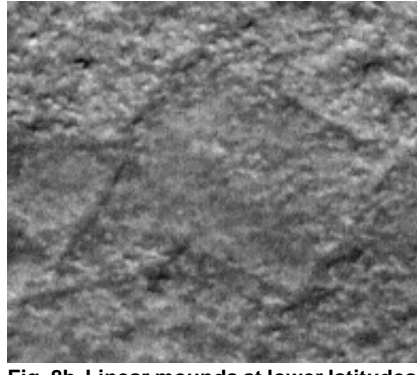
Fig. 8b Linear mounds at lower latitudes.
