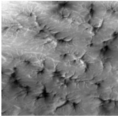
Fig. 1b Spiders – with branches (tubes) above ground. Some may have a ravine core, others have a mud-like core.
