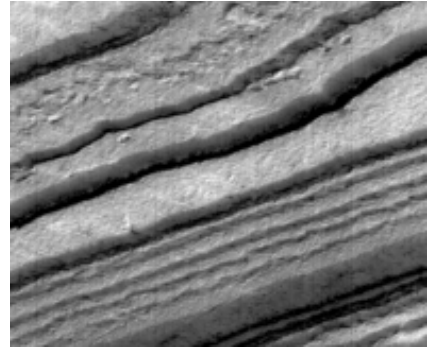
Fig. 4c Alternate dark albedo tuff-like bands undercut ice layers.
