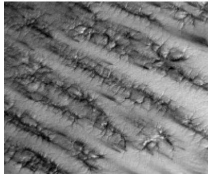
Fig. 1h Branch (creeper) forms of spiders adopting the joint pattern of the host rock. These look like normal creek systems when inverted. Scale: ~1.10 km across image.
