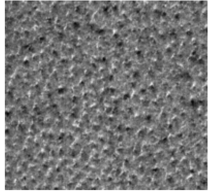
Fig. 7f 36.67°W, 76.82°N. Compare this platform comprised of old-tree (stump) shapes from the North Pole, with M0808054 (192.70°W, 77.90°S), from the South Pole. Both have almost identical texture. Scale: ~2.8 km.
