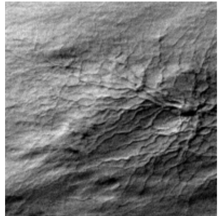
Fig. 1c Spider with a central mud-like core. Several legs display meandering patterns – normally attributed to flow of a liquid such as water. There is some jointing control of the branches (legs) in the bottom of the image.
