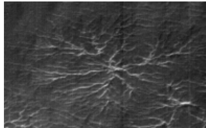
Fig. 10c 262.65°W, 85.80°S. Inter-growing spiders, 700 m across, with mud-like core; untouched. The reader should try to fit the fibonacci pattern. Note the similarity of the Fig. 8i toe area to the branch ends.
