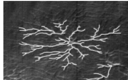
Fig. 10d 262.65°W, 85.80°S, A different spider shape (800 m across) from the same area with fibonacci-type pattern outlined.
