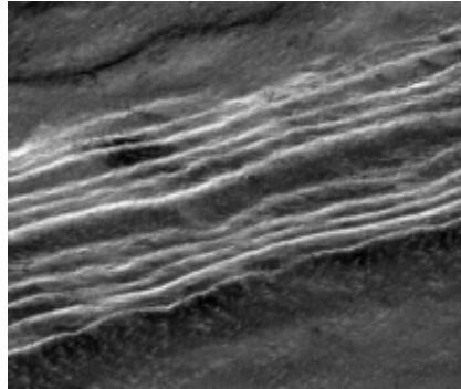
Fig. 5b Layers forming terraces.
