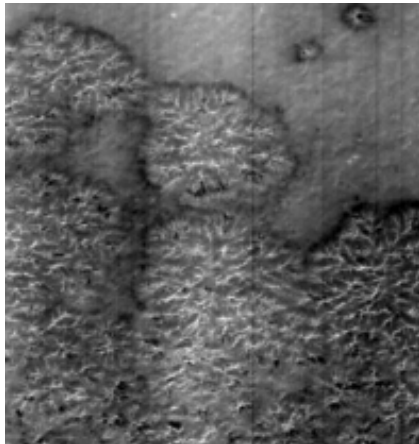
Fig. 1g 284.38°W, 82.02°S. Scale 2.83 km across. Bush or Banyon Tree structures.
