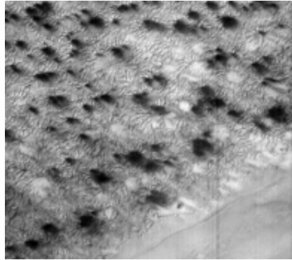
Fig. 2h 192.70°W, 77.90°S, Scale: 2.85 km across image. Spring. Amoeba shapes on a large terrace. Sand or ice tends to collect around/between the amoeba as they create a sand-like terrace.
