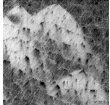
Fig. 8c 107.95°W, 86.16°S. Scale: ~1 km wide. Spring. Large fans from the South Pole forming terraces of alternate dark and light coloured material.
