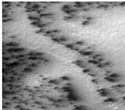
Fig. 5h 290.05°W, 80.78°S. 2.4 km wide. Late winter. Fans and ravines adopt the bedding planes. Cross cutting faults are avoided.
