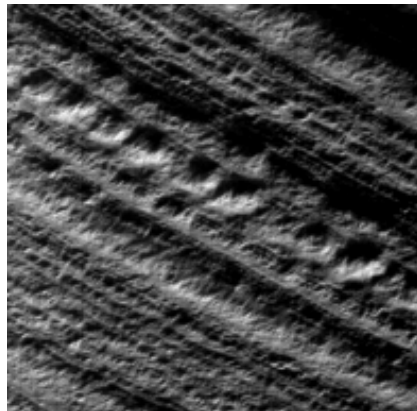
Fig. 4d A pitted texture with remnant tubes and ravines. Our interpretation is that large fans created through cross-bedded (TCB) terraces (see Fig. 8). This image (and the others) may represent the same TCB units etched or eroded by the process of retreat – caused by the growth of tubes and ravines related to specific (dark albedo) layers.
