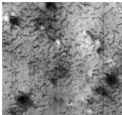
Fig. 9e 179.29°W, 75.77°S. Scale 2.2 km across image. A platform with rotated and pitted forms in mud-like material at the South Pole. The vent (hole) on the left has burst. Note the small-rotated starfish shape above this. The serrated and pitted textures are hard to explain geologically. On the right side is a mud volcano. A serrated spiral form exists in the top right side of the image. The sponge shapes are probably small vents. There may be water near the surface.
