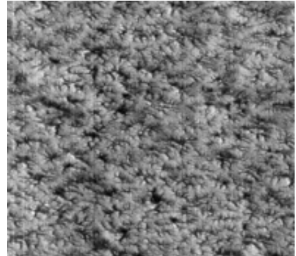
Fig. 2i 224.26°W, 77.01°S, Scale: 2.6 km across. Ravines, each ~200 m in size, venting dust and basalt (or mud-like). The platform surface texture mimics large mud-cracks.
