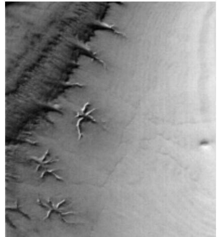
Fig. 2f 177.45°W, 76.88°S, Scale: 1.4 km across image, so objects are ~250 m across. Squid-like shapes are attached to the dark tuff (?) band (the flat body area may be dust/mud jets?). Five legged (unusual for geology) star fish or tree shapes. The mud-like layers are probably retreating, which allows fluids to become available so the structures can form.
