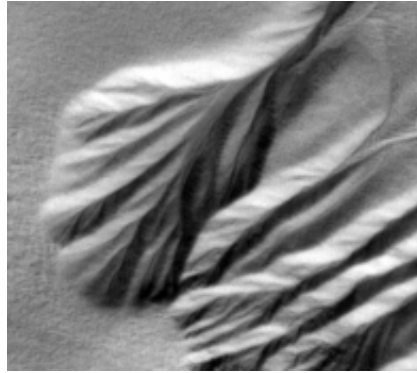
Fig. 8h The same pattern at 60°S. The fluid seems to be expelled at the top or along the ends.
