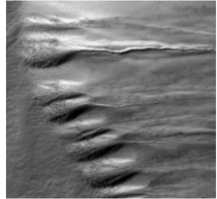
Fig. 8i A variant with long feeder tubes (if the sand/ice cover was melted we would see an open canyon). Note the slight meander of tubes and the way the fans have formed ridges – so this may be growth rather than retreat. The small spots in the dune toe may be small fans and the gray albedo on the left is probably dust or gas.
