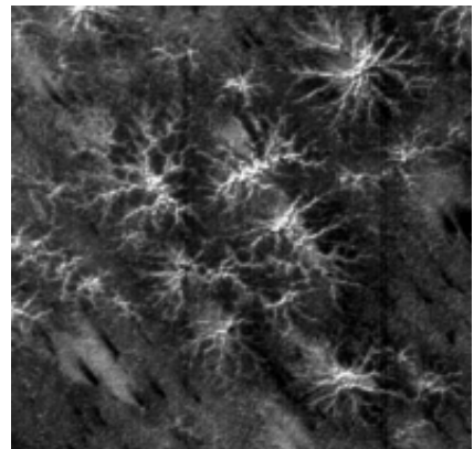
Fig. 1f 273.96°W, 86.96°S. Scale: Spiders are ~200 m across. Spring. Spiders with either a hollow or a mud-like core or plug. The dark linear areas are fans. The elongate areas of pale albedo are probably ice/snow. Ice/snow is deposited between spider branches.
