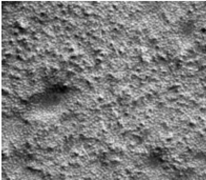
Fig. 7d 77.78°W, 59.91°S. Scale: 1.41 km wide. An ancient spider terrace, with a honeycomb texture of overprints. The texture where two holes are aligned (like a pair of eyes) is common – each is an opposing vent from an old spider. The parent image has craters impacted onto the platform.
