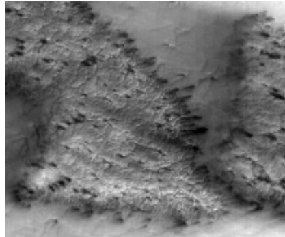
Fig. 7b 178.98°W, 75.63°S. 2.8 km wide. Spring. A raised platform created by spiders, with tubes forming on the edges. Spider platforms tend to avoid depressions or bend around craters. There seems to be a crater on the left side of the platform (due to the curve).
