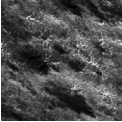
Fig. 7a Amoeba and spiders form complex inter-growth patterns.
