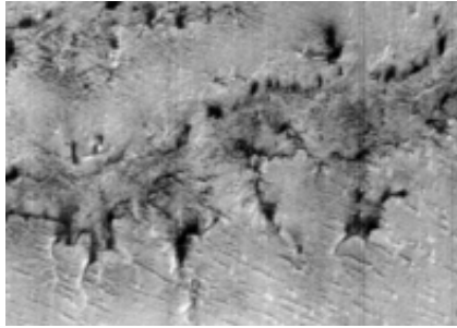
Fig. 2g Mud-like material forms a central pack. This image may also contain outflow channels formed by bursting of spider branches.
