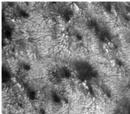
Fig. 1d Linear (elongate) mounds infill the joints. Complex structures form from mud-like cores at the intersection of the joints. Scale ~1.5 km across.
