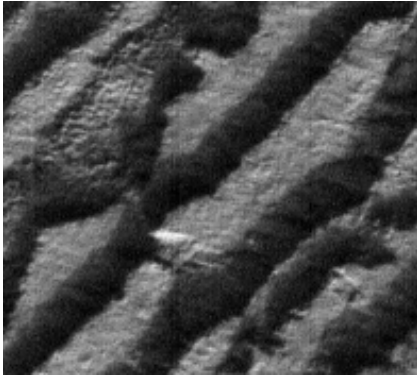
Fig. 4a 184.39°W, 86.67°S, Scale: ~200 m across. Dark albedo layers in the top image are tuff-like bands that may have oozed material out of the bedding plane. It looks like plant matter but may be a CO 2 gas plume (?). It is unlikely that layers could 'grow' to form a uniform thickness. The collapse structure indicates the macro bands are retreating.
