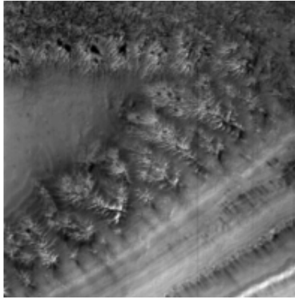
Fig. 2a 157.39°W, 76.57°S, Scale: 2.8 km across image. Terraces (forests) of branch (creeper) forms, confined to one rock type. Sand/ice/snow deposits fill gaps between spiders.
