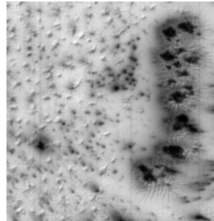
Fig. 1i 69.94°W, 73.59°S. Spring. Scale: ~1.4 km wide. On the left: small joint controlled amoeba with a central core and numerous legs. On right: larger Amoeba shapes with a dark core and more complex tubes radiating from the large central core/fissure. Dark albedo material is deposited over the branches. Note the small dark fans associated with the structures.
