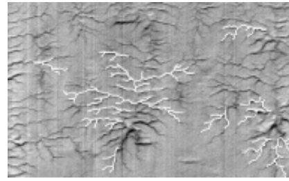
Fig. 10b The same branch image showing the fibonacci-type pattern outlined.
