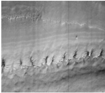
Fig. 9a Terraces in retreat. Spider tubes form perpendicular at the base of layers.
