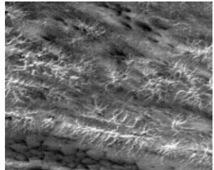
Fig. 5i 268.57°W, 87.00°S. Scale: 2.85 km across. Three-dimensional views showing terrace layering. Gas and fluids expelled take the shortest path to the surface – up any joint or crack (in cliff).
