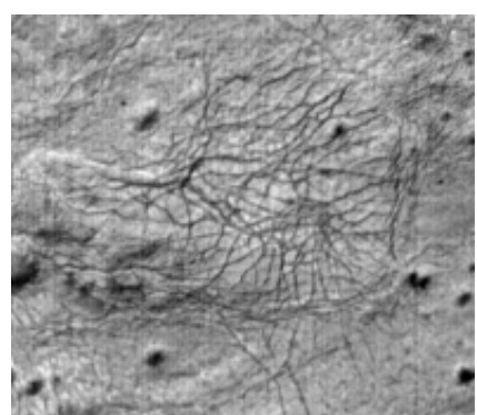
Fig. 2l A spider from a non-polar area, Southern Hemisphere. The spider legs are fine and growth extends from one single limb, but tends to cross more randomly than other complex spiders (may be a result of resolution).
