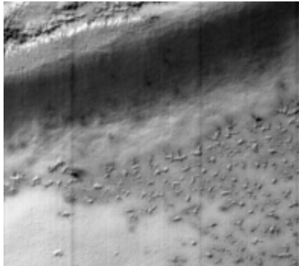
Fig. 2j 34.96°W, 77.47°S. Late Spring. Spiders, each ~200 m across, are in a large circle (lower right of image), so are venting up the side of an old impact crater. The largest one in the center has a mud-like (?) core. This follows the pattern of magma – but they mimic mud volcanoes.
