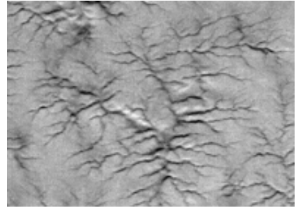
Fig. 2c A spider in winter with a mud-like core.
