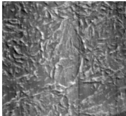
Fig. 7e 132.79°W, 31.61°N. Scale: 1.6 km wide. Old terrace of ravines/spiders from the equator. They have pale albedo infill as with spiders. The creeks are not inter-linked and seem to join at a central point – as with ravines or spiders.
