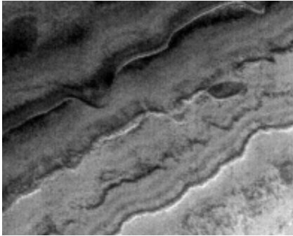
Fig. 5a 230.26°W, 77.48°S. Scale: 2.12 km across. Mudslides – in thick tuff-like beds implies saturation by a liquid e.g. water.
