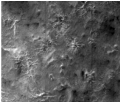
Fig. 1a 151.62°W, 87.10°S. Fans (dark) with two directional orientations (top left). Spiders are pale albedo, typically with a mud-like core. The image is ~800 m across. Small pockmarked spots or hollows in the image are older or non-active - this is what the fans look like in ancient terrain (i.e. pockmarks or etched terrain). Several small light-coloured (raised) mounds in the middle and lower right of the image have one single (one-armed bandits) or two small rotating arms.
