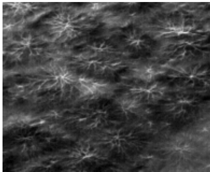
Fig. 1e 291.44°W, 83.10°S. Three-dimensional Martian Boab-tree structures above plain level, surrounded by small spiders. The large objects are 200 to 400 m in diameter. Some have a hollow and others a solid core (pale albedo).
