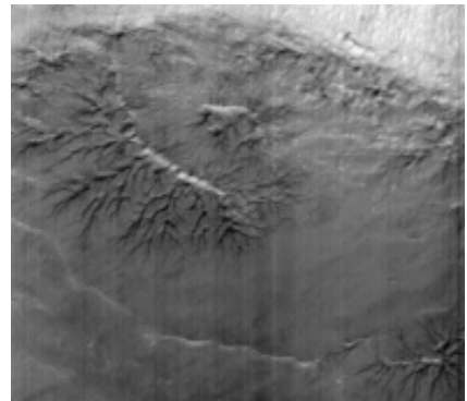
Fig. 9f Spiders that look much like a plant root system. The top layer slid down to the left breaking the original spider branches (on the top of the layer) – the reader can rejoin them. There are also spider tubes growing from the layer at the base of the bedding plane etching the planar fault.
