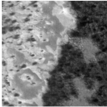
Fig. 9b The dark albedo (black 'blob') material on the right forms bush-shapes with feeders being permafrost fractures. The area on the left either represents different underlying rock or subsurface depletion of source fluid from layers.
