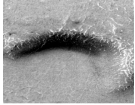
Fig. 7c 7.81°W, 75.63°S. The spider terrace is some 1.42 km across and over 50 m thick. This shows that spiders create a large thickness of vertically stacked spider terraces. The terraces are undercut. The curved shape may be due to avoidance of an old crater.
