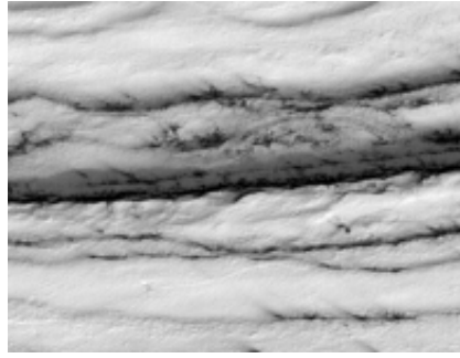
Fig. 4b 21.24°W, 84.16°S. Scale: 2.13 km across. Parallel tuff-like bands in the bottom image adopt negative relief creating ravines. Dark mud-like material has covered the bands above and below the venting mud-like layer. The image has captured a turbidity flow of ice/mud mix being ejected from a central vent (semi-circle structure due to the effect of gravity and the slope) like an avalanche.
