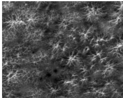
Fig. 2e 265.49°W, 87.13°S. Scale: 2.4 km wide. Spring. Large complex spiders several hundred metres across surrounded by small ones. The spiders tend to follow the pattern of the underlying rock, which indicates that this platform is relatively thin, therefore may also be fairly young, supporting the observation that platforms may be created in a single season.
