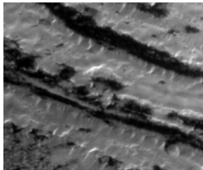
Fig. 2k 304.68°W, 81.35°S. Scale: 1.42 km wide x ~1.0 km high. The parent image shows folded beds and ravines/fans developing and undercutting in specific layers. The dark 'blob' material looks like a plant but may be CO 2 and other minerals venting.
