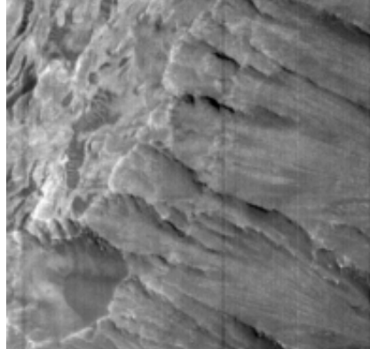
Fig. 8d (left), 8e (middle) and 8f (right) 62.08°W, 3.74°S. Each ~1.74 km wide. Late spring. Trough-cross bedded (TCB) terraces of light and dark material have formed from venting of material (possibly clathrates or ice and eroded bedrock minerals) via faults. The beds are not folded; it is the same rock unit in a continuous sequence.
