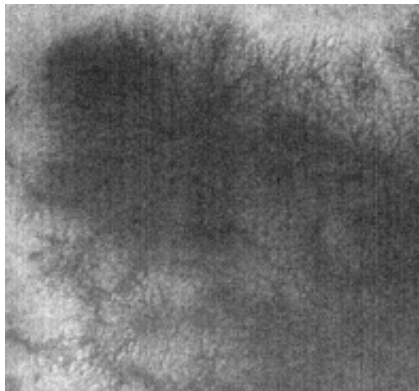
Fig. 9d A similar object, which may be cryptic CO 2 growing along cracks in the ice.
